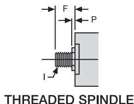
THREADED SPINDLE
