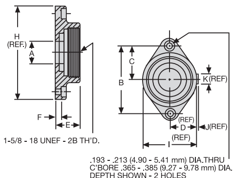
37893 FLANGE MOUNTING BRACKET
