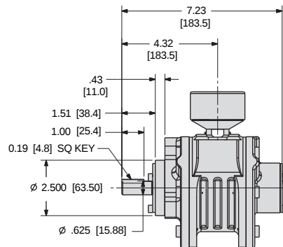
SM6AMA and SM6AM-AH636 FOOTMOUNT DIMENSIONS
