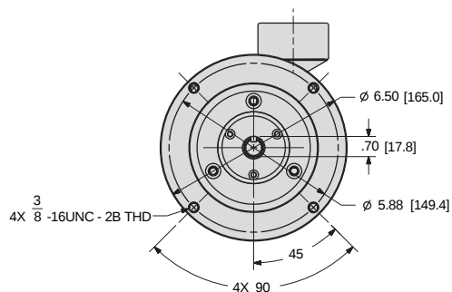
SM6AMAN NEMA MOUNT DIMENSIONS
