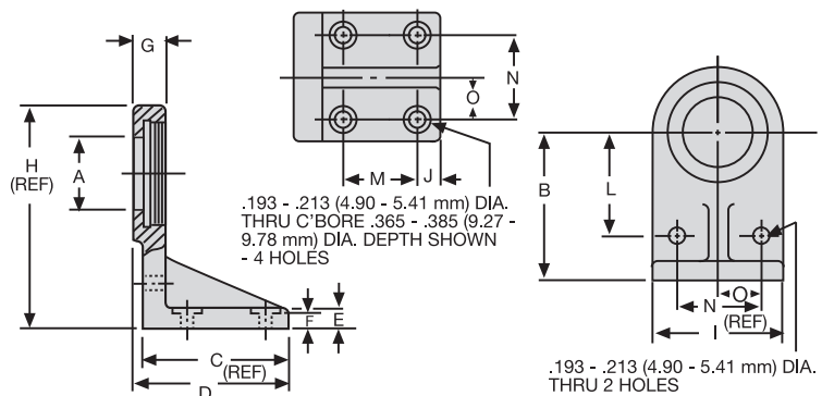
37897 FOOT MOUNTING BRACKET
