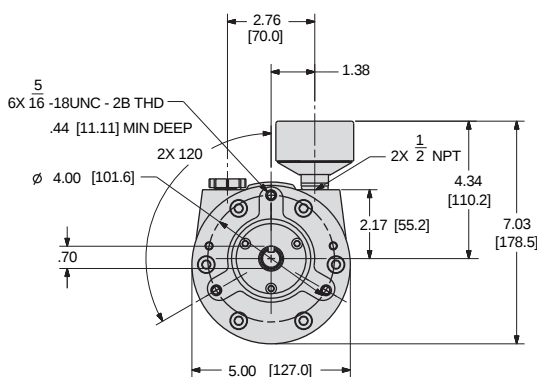
SM6AMA and SM6AM-AH636 FOOTMOUNT DIMENSIONS
