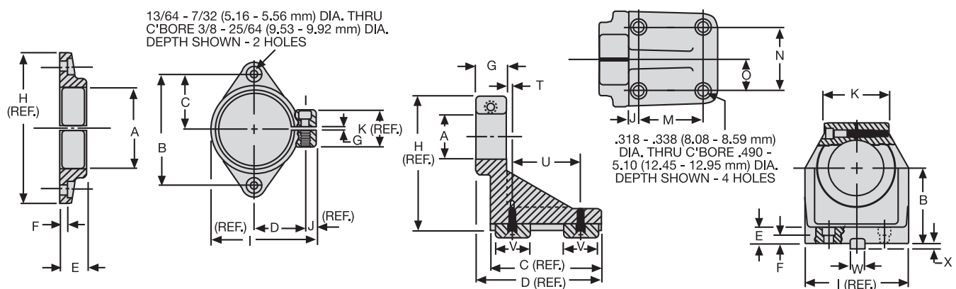
41559 FLANGE MOUNTING BRACKET
