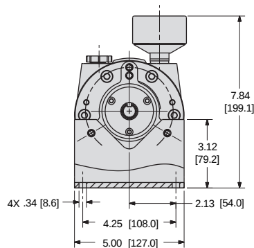
SM6AMAN NEMA MOUNT DIMENSIONS
