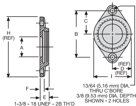
37896 FLANGE MOUNTING BRACKET
