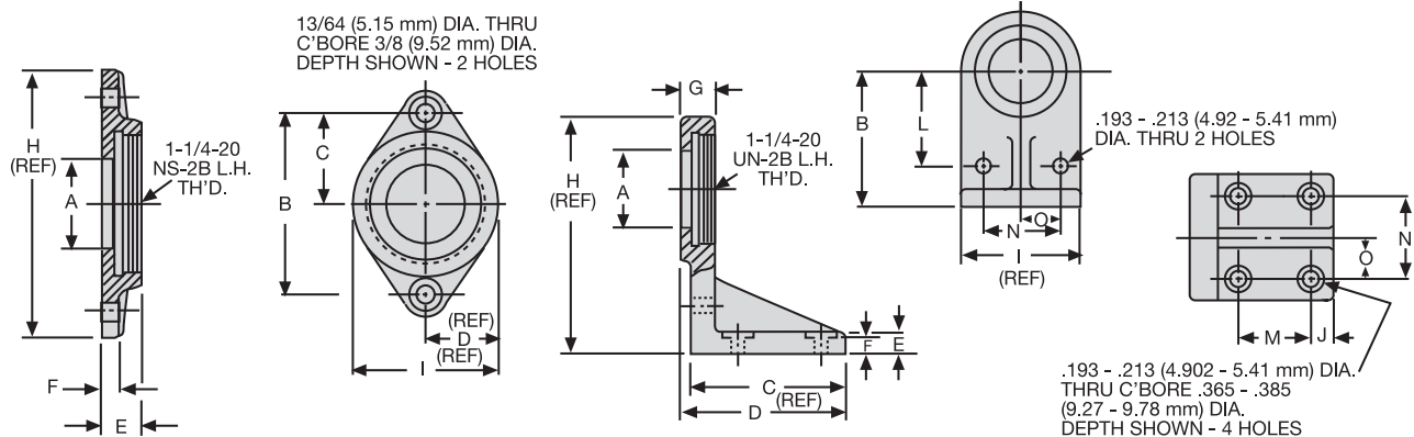
37898 FLANGE MOUNTING BRACKET
