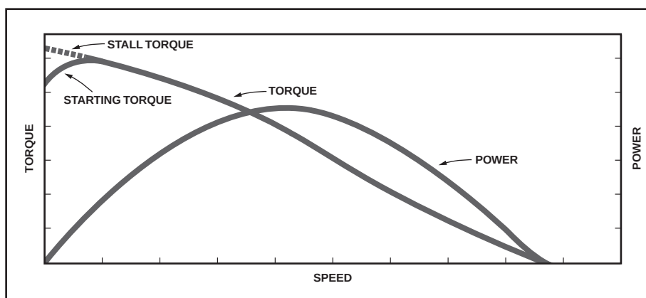
Fig. 1. Torque and power curves for a typical air motor. Torque is maximum at zero speed and zero at free speed. Any loading will slow the motor. As the load increases, the speed decreases and the torque increases until the motor stalls. If the load is decreased, the motor speed increases and its torque output decreases to match the applied load.
