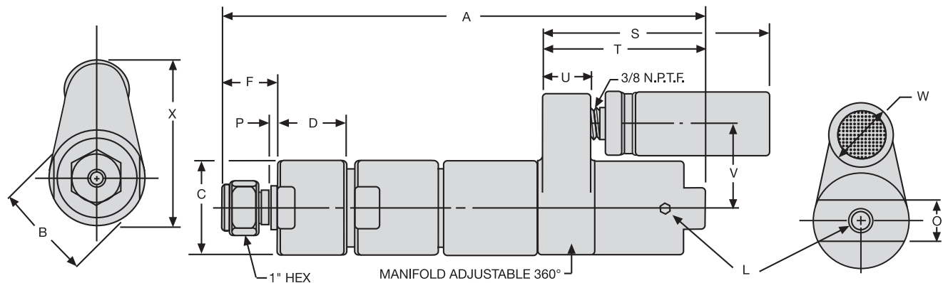
FORWARD ROTATION, DOUBLE REDUCTION SHOWN
