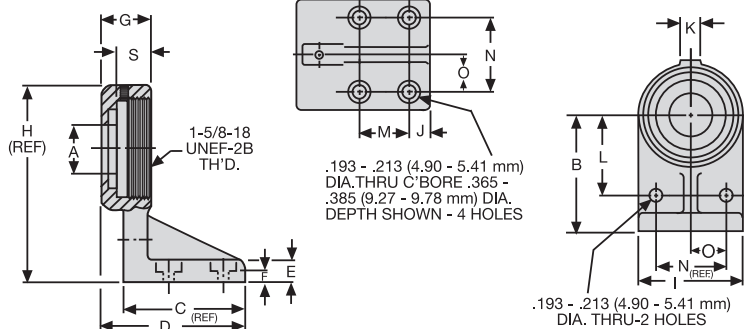
37894 FOOT MOUNTING BRACKET
