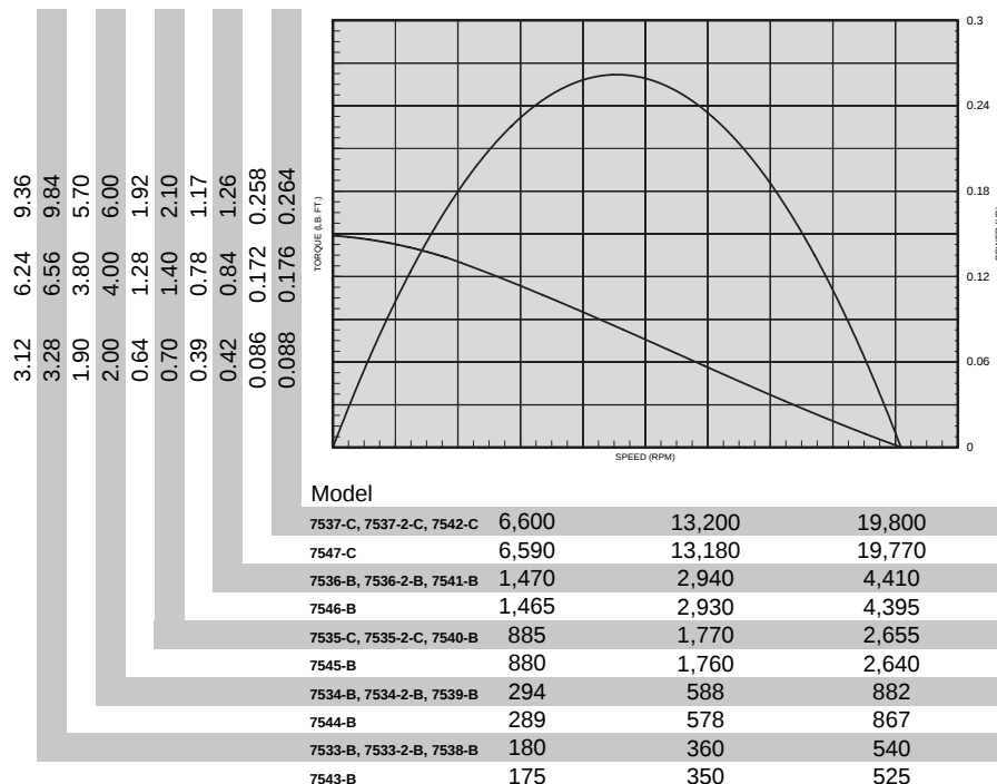
Approx. Tooling Penetration - 1 1/8" (28.6mm)
