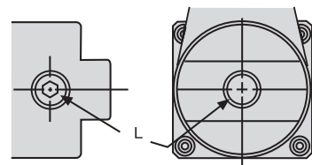
AIR INLETS, SINGLE DIRECTION MOTORS
