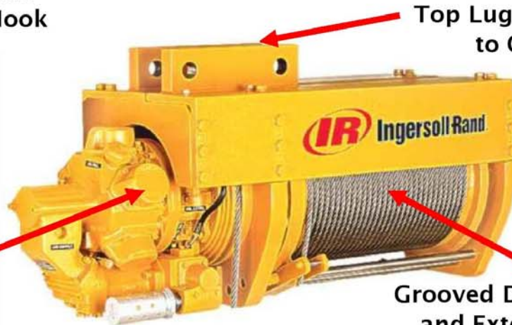
Heavy Duty Radial Piston Air Motor
